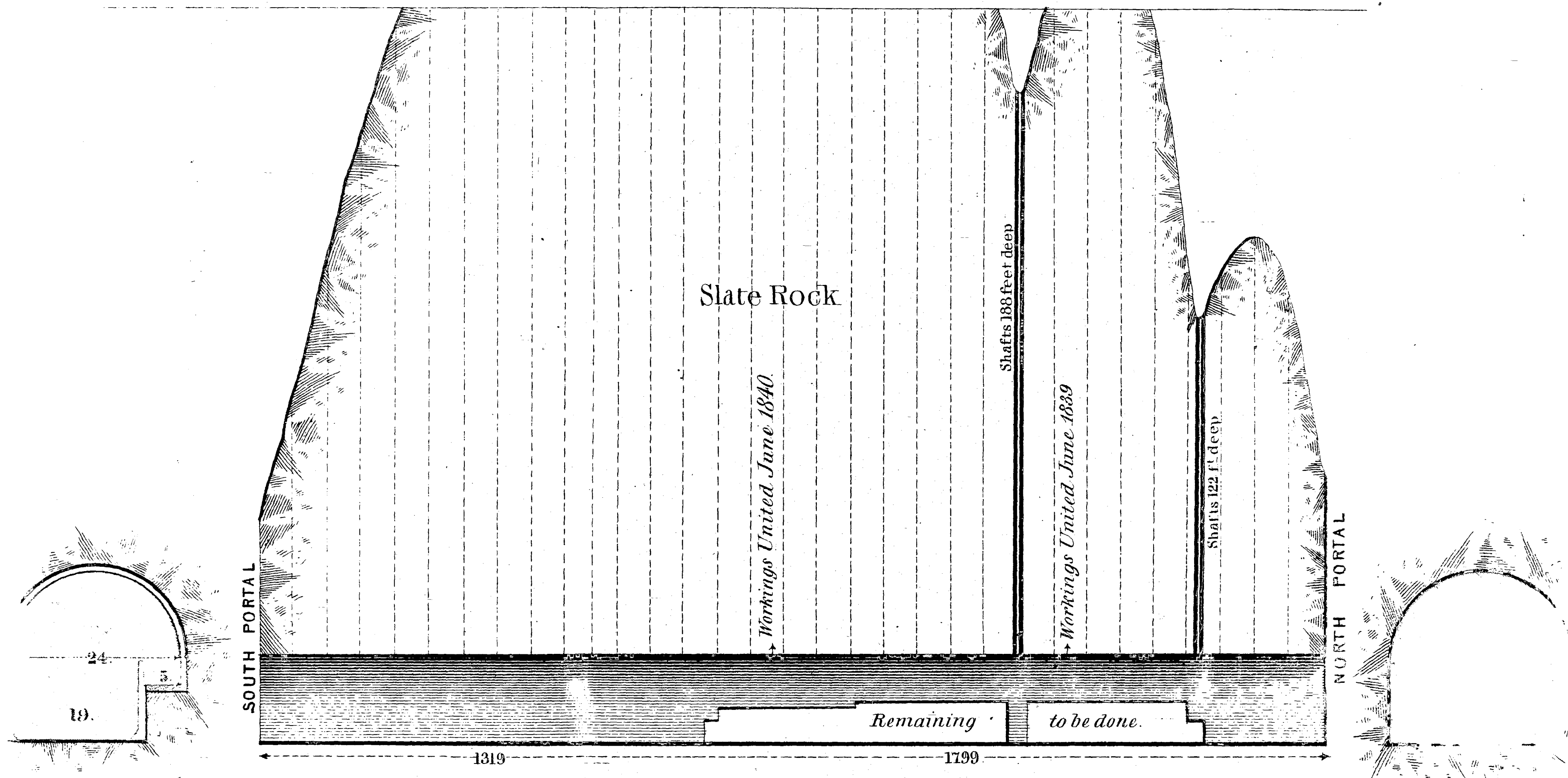
Fig. 1. Tunnel 3118 Ft.
