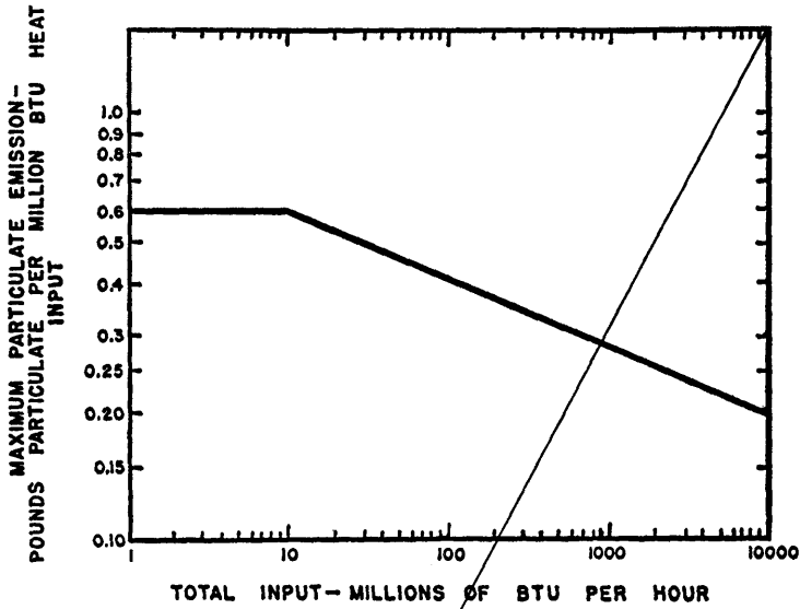
Figure 2 Maximum Emission of Particulate Matter from New Fuel Burning Installations
