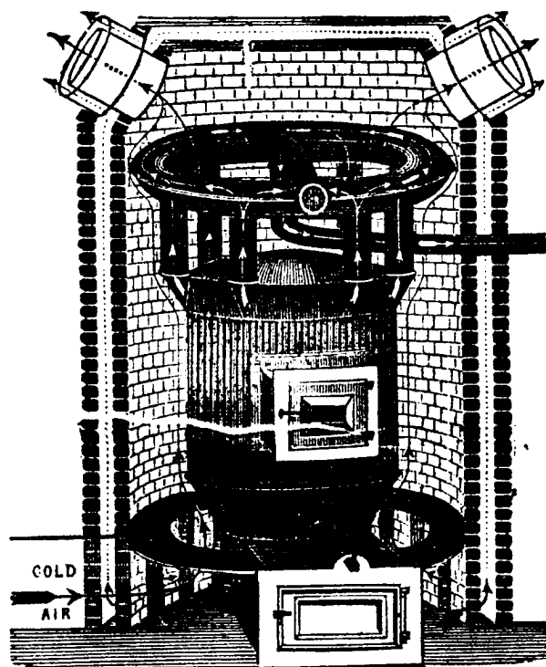
Chilson's Air Warming and Ventilating Furnace.
