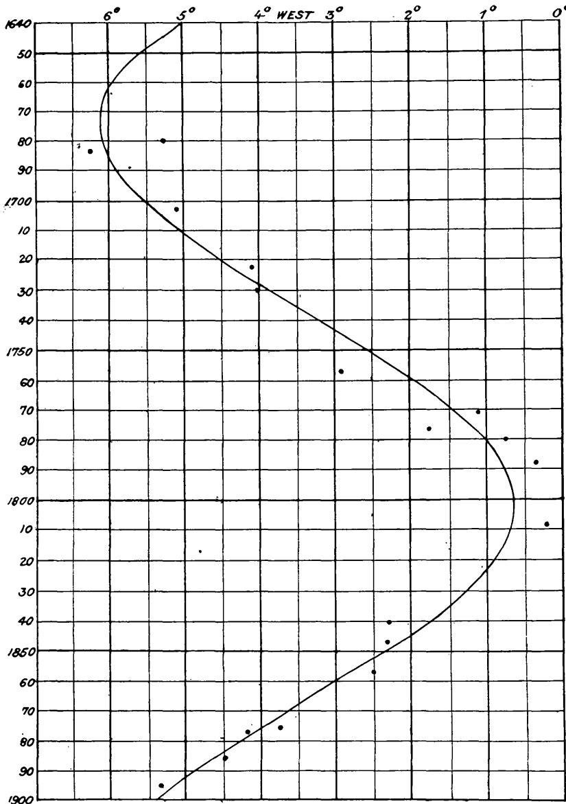
FIG. 6.—Illustrating the secular variation of the magnetic declination at Baltimore. The curve represents the values computed according to formula and the dots represent the observations.
