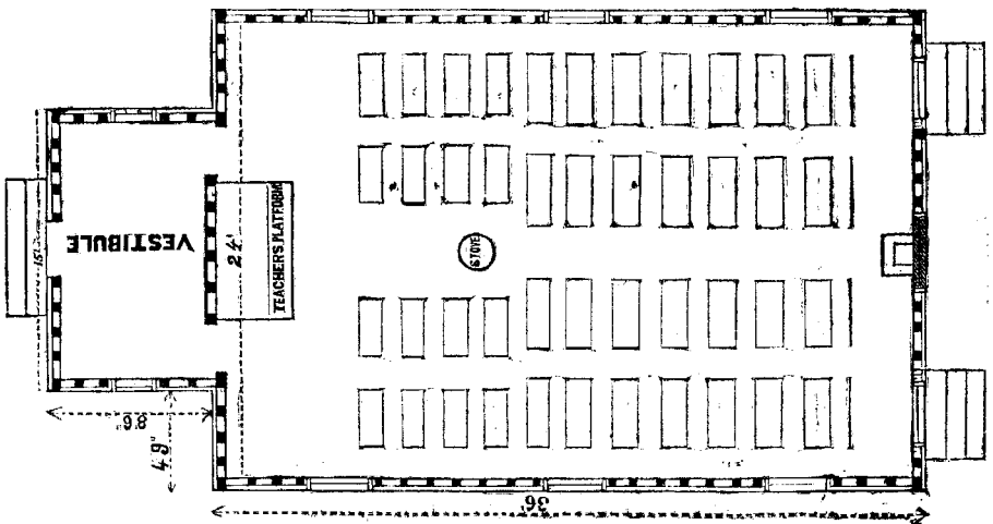
Ground Plans of Nos. 2, 3 and 4.
