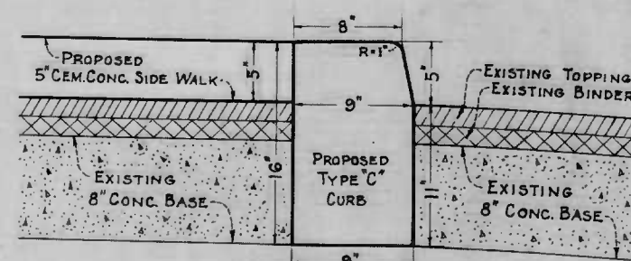
TYPE "C" CURB
