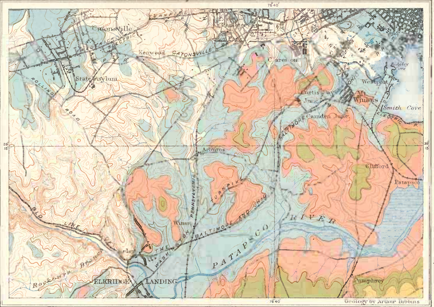
MAP SHOWING AREAL DISTRIBUTION OF CLAY-BEARING FORMATIONS OF THE POTOMAC GROUP IN THE REGION SOUTHWEST OF BALTIMORE CITY
