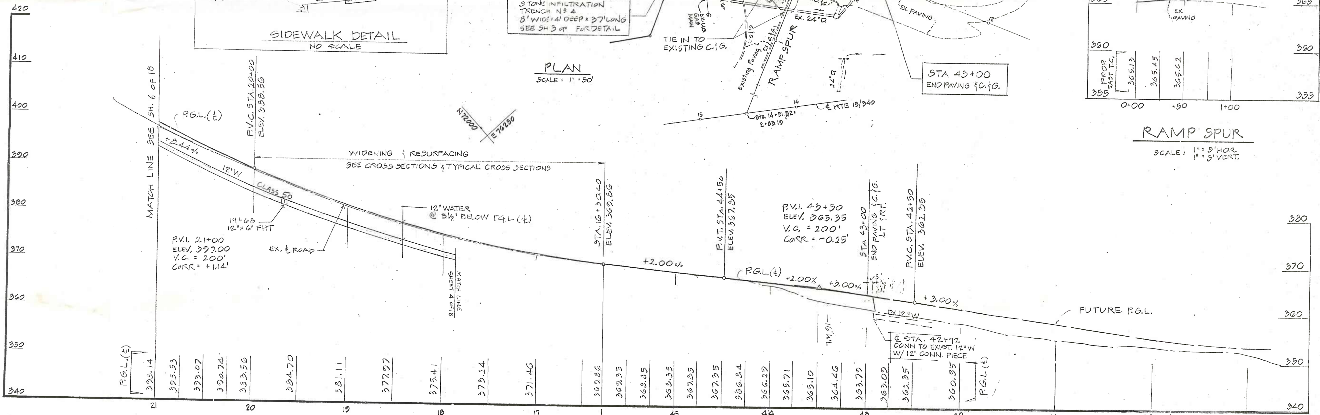
PROFILE SCALE: 1"=50' HOR. 1"=10' VERT.
