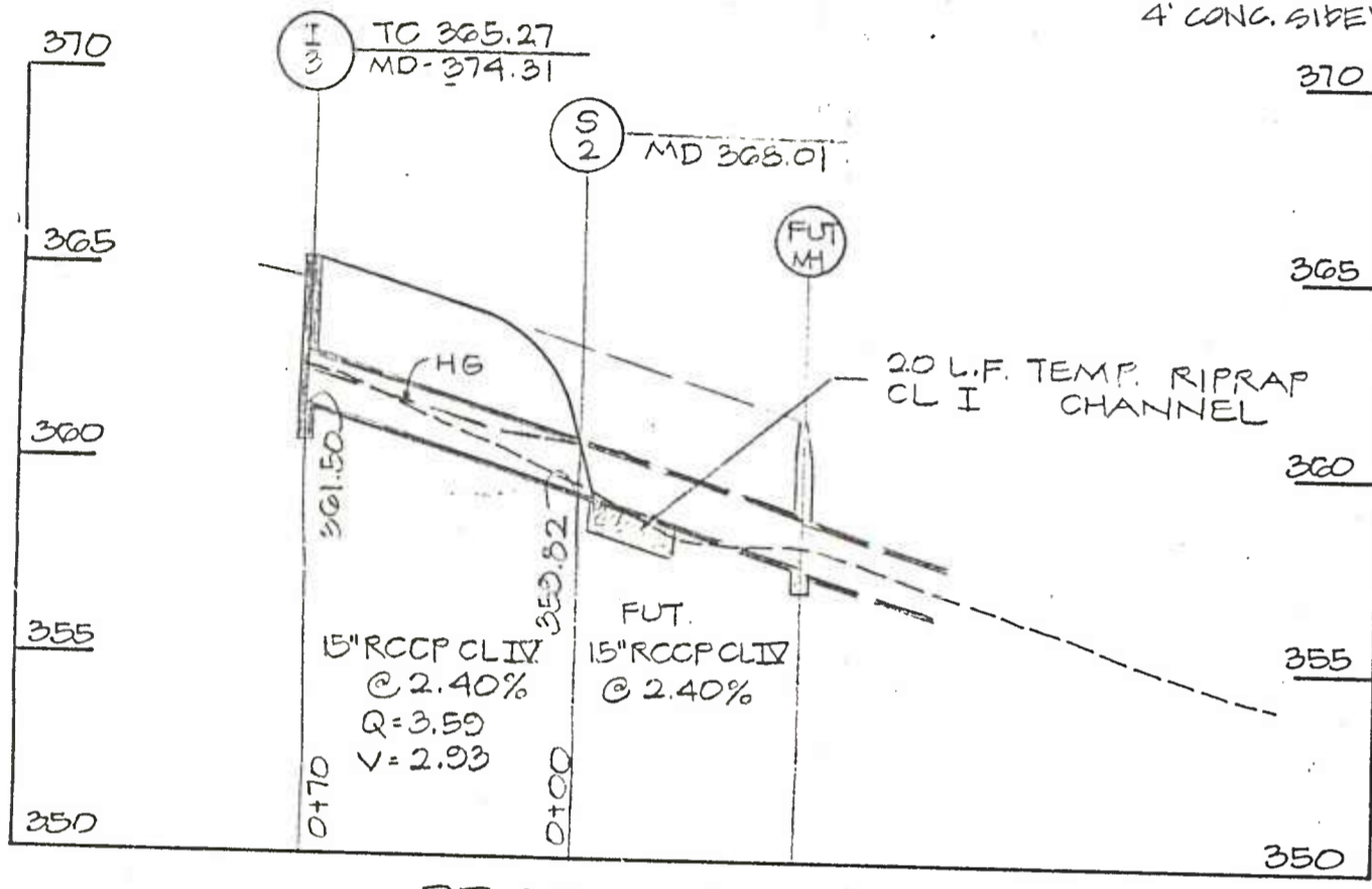
PROFILES SCALE: HOR. 1"=50' VERT. 1"=5'
