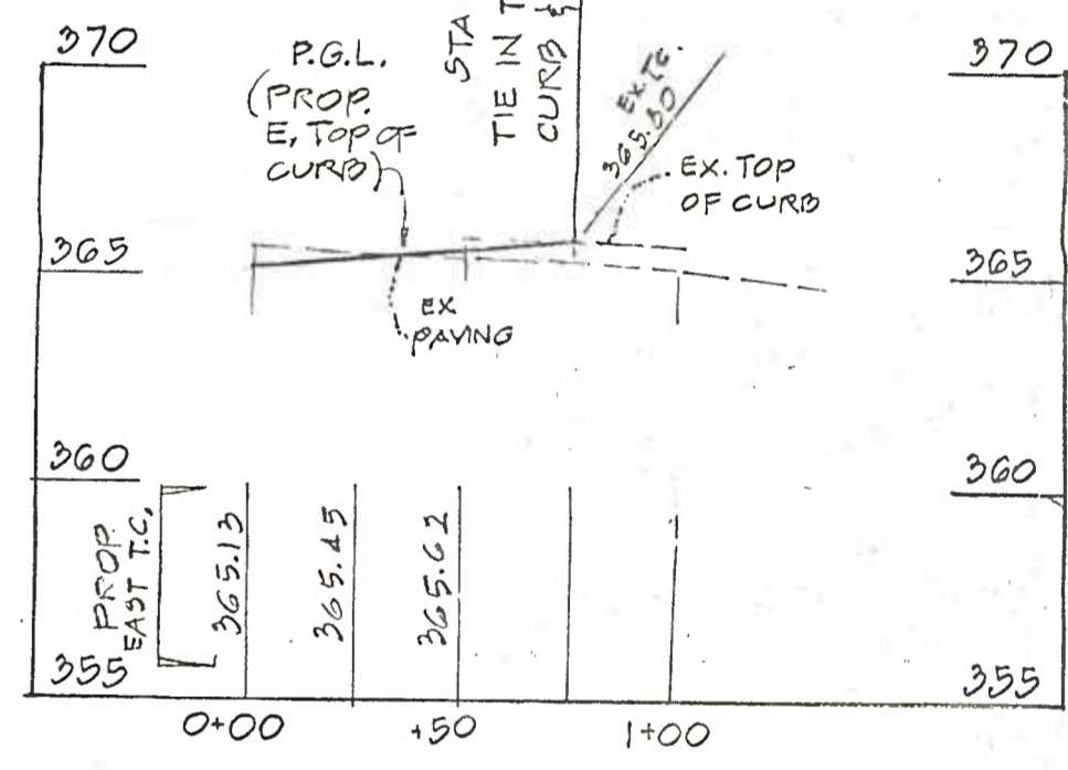
RAMP SPUR SCALE: 1"=5' HOR. 1"=5' VERT.
