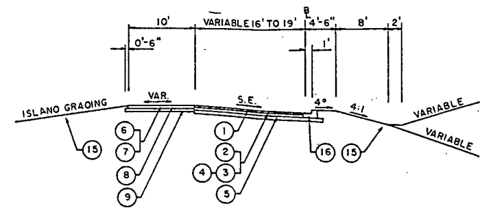
RAMPS - CURVE SECTION RADIUS LESS THAN 400 FT.
