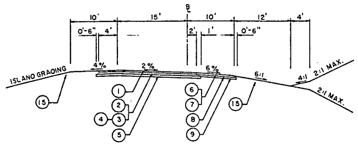
RAMPS - TANGENT SECTION
