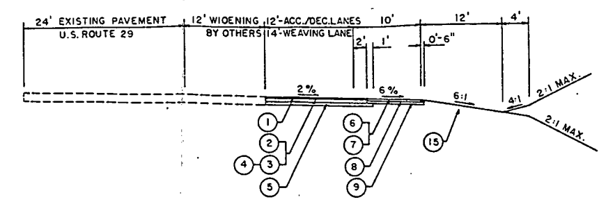
RAMP ACCELERATION & DECELERATION LANES
