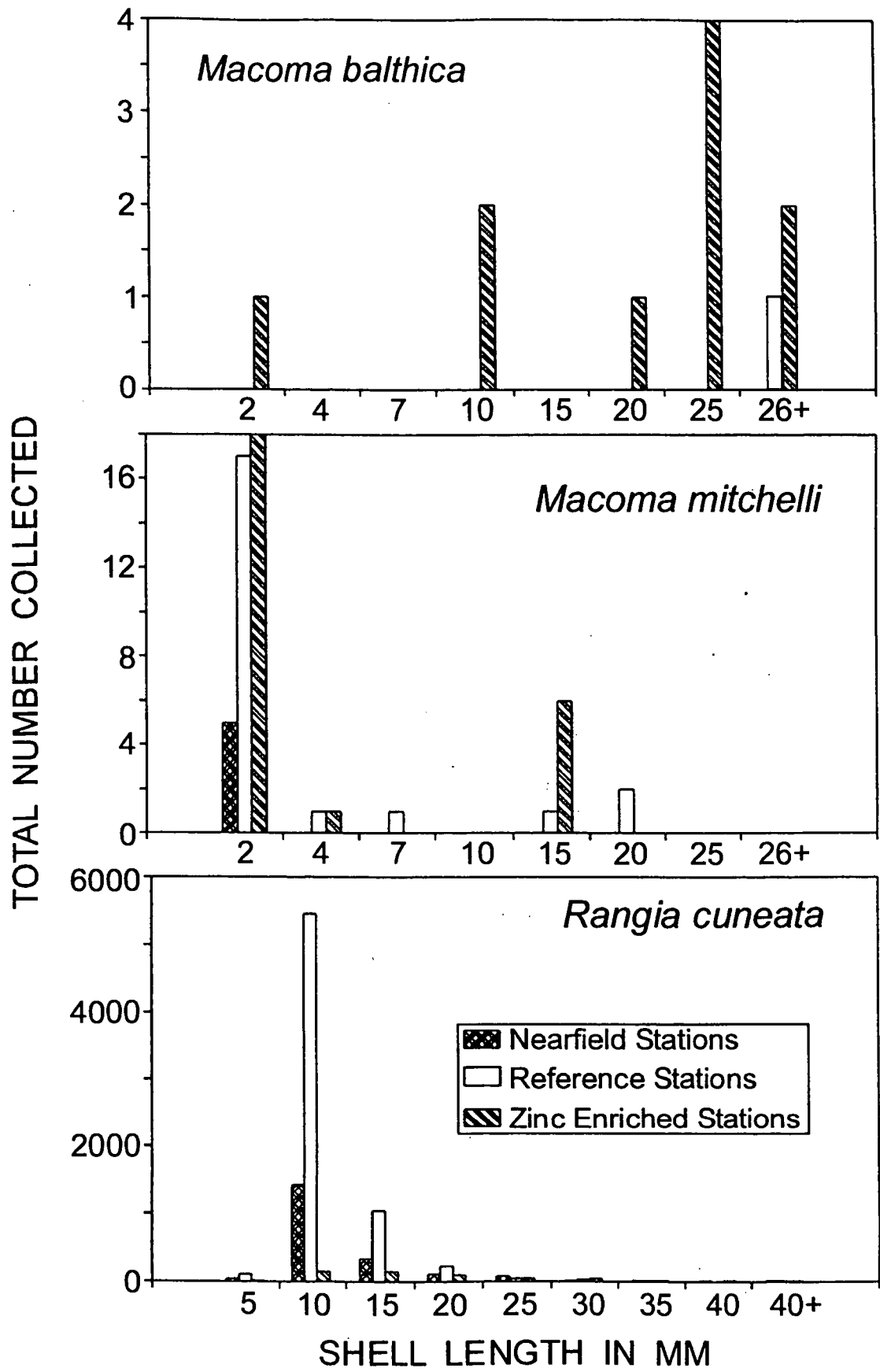
Figure 3-2. Length frequency distribution of the clams Macoma balthica , Macoma mitchelli , and Rangia cuneata during the 16th year of benthic monitoring studies at HMI.
