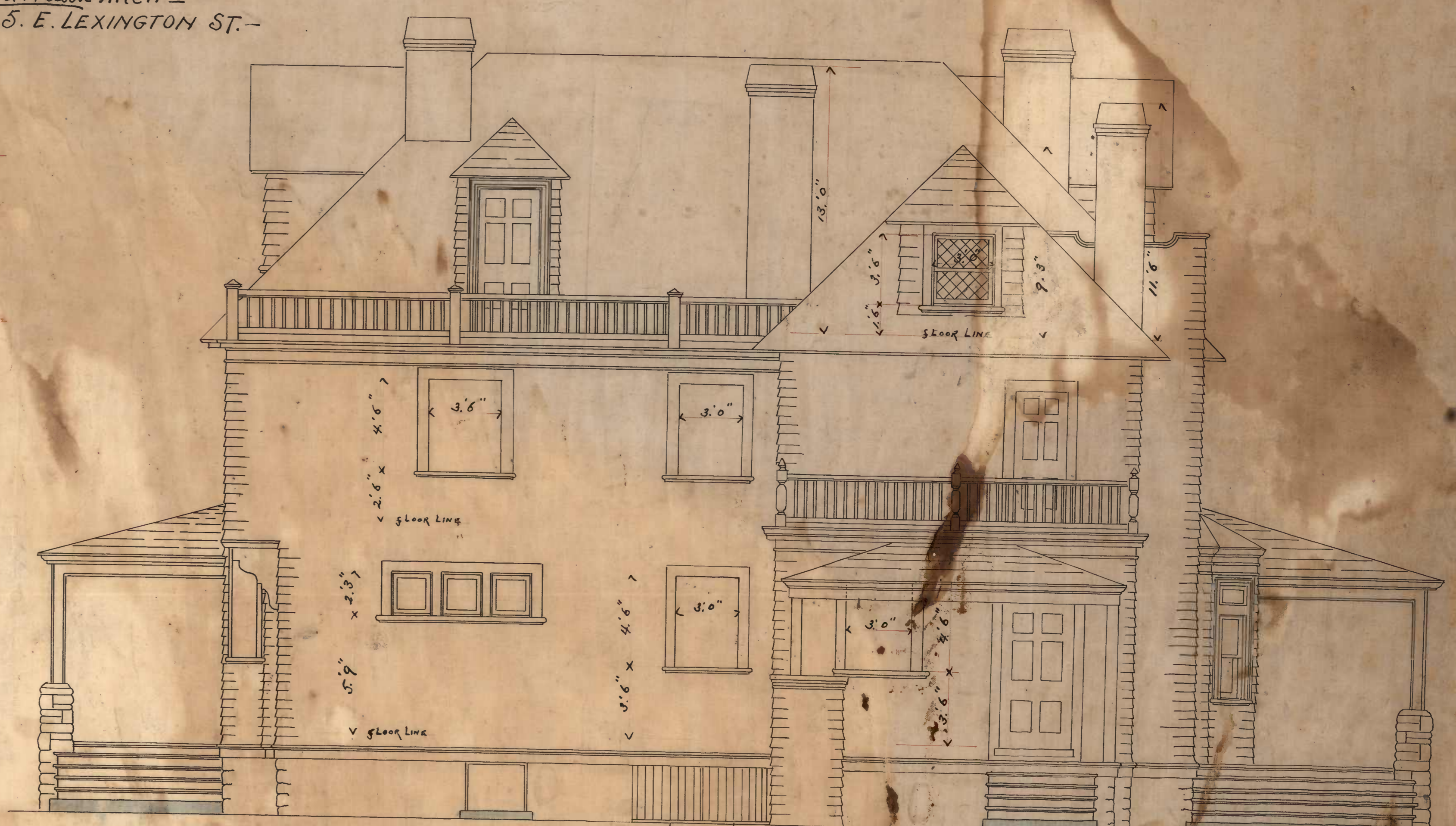
- EAST ELEVATION -
