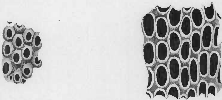
FIG. 10.—Portions of the surface of Membranipora parvula . \times 22 .
