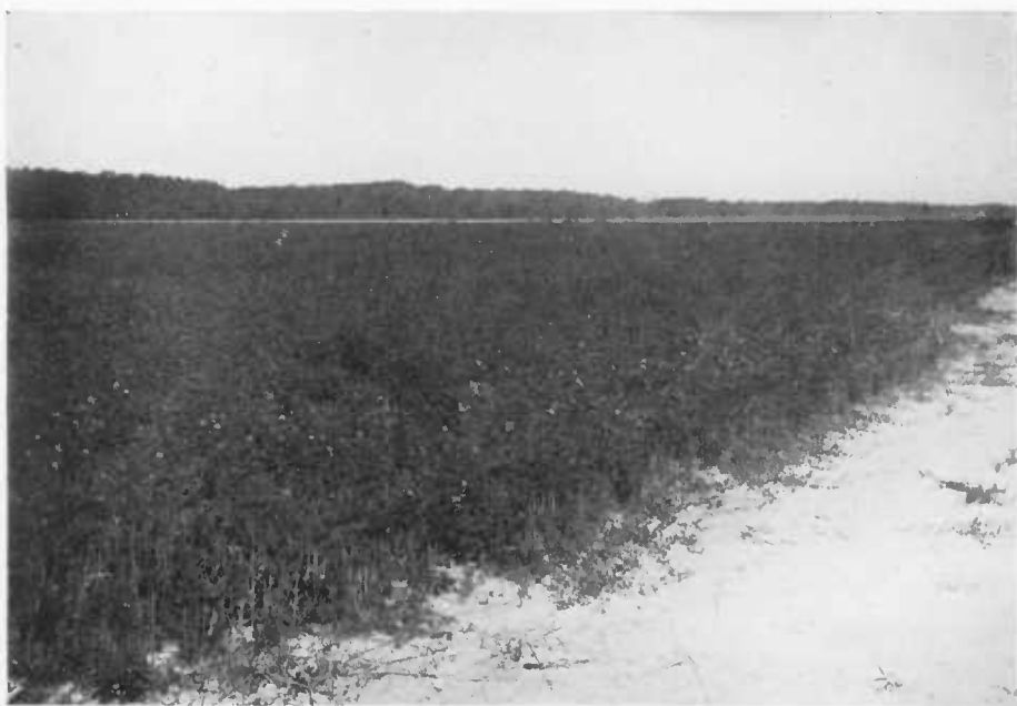
FIG. 2.—VIEW OF TALBOT SURFACE, NEAR TAYLORS ISLAND, DORCHESTER COUNTY.
