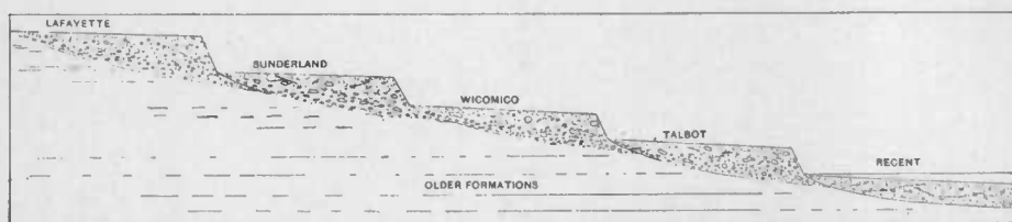
FIG. 2.—Diagram showing ideal arrangement of the various terrace formations in the Maryland Coastal Plain.
