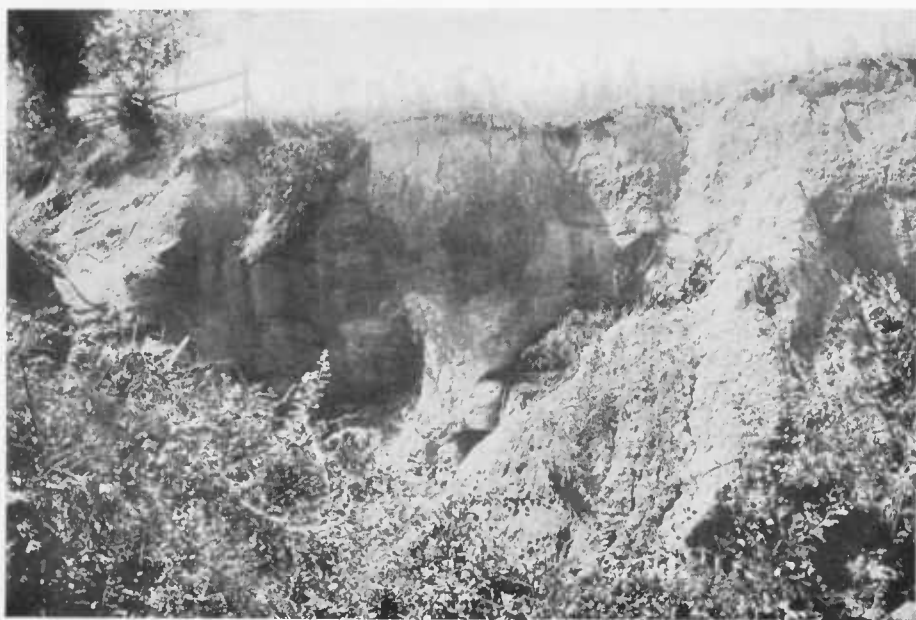
FIG. 2.—VIEW SHOWING SECTION IN SUNDERLAND FORMATION AT RIDGE, ST. MARY'S COUNTY.
