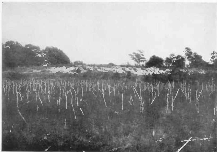
FIG. 2.—VIEW SHOWING SUNDERLAND-WICOMICO SCARP, WICOMICO SURFACE IN FOREGROUND, NEAR LEONARDTOWN, ST. MARY'S COUNTY.
