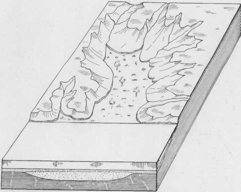
FIG. 7.—Diagram showing advancing Talbot shore-line and ponded stream.
