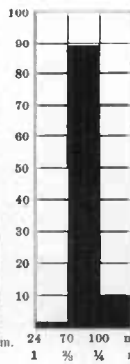
K.—Dune at mouth of Indus. Oldham.
