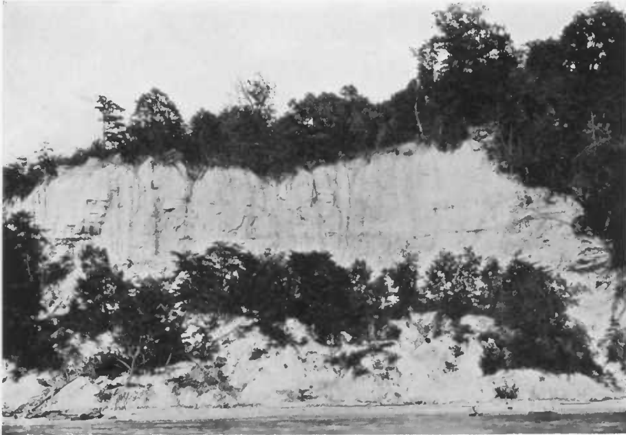
FIG. 1.—VIEW OF LOWER WHITE BANK, FLK NECK, SHOWING PATAPSCO, RARITAN, AND MAGOTHY FORMATIONS.
