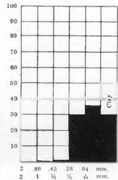
I.—Sample 9. Matawan formation, Grove Point.
