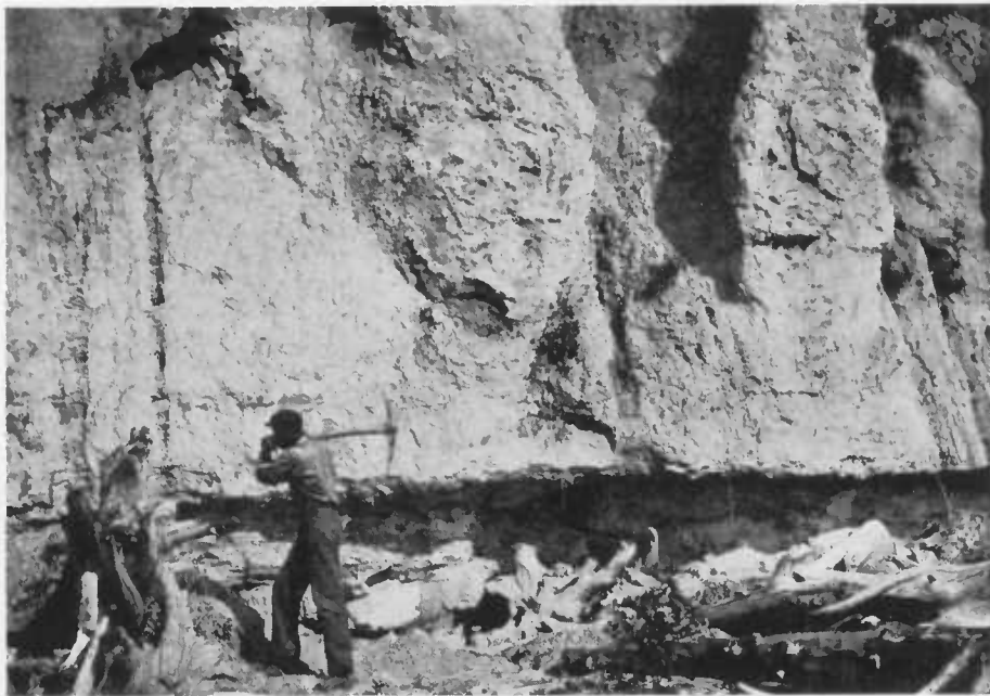
FIG. 2.—VIEW OF GROVE POINT SHOWING MAGOTHY FORMATION OVERLAIN BY MATAWAN FORMATION.
