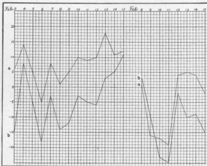
FIG. 11.—Minimum temperatures during the cold waves of February, 1895, and 1899, at—(a) Charlotte Hall, (b) Deer Park.
