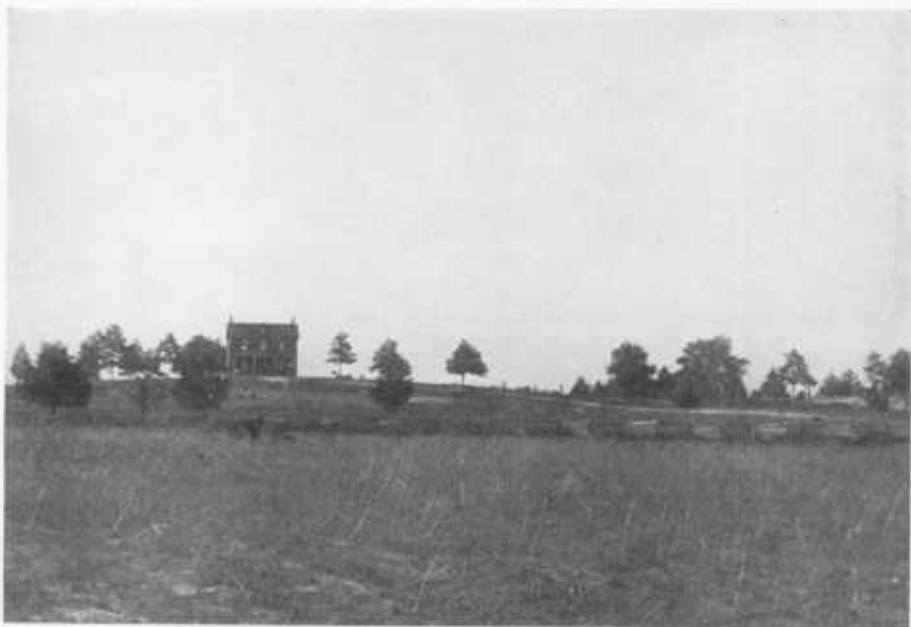
FIG. 1.—VIEW SHOWING LAFAYETTE-SUNDERLAND SCARP, SUNDERLAND SURFACE IN THE FOREGROUND, CHARLOTTE HALL.
