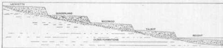
FIG. 4.—Diagram showing ideal arrangement of the various terrace formations in the Maryland Coastal Plain.
