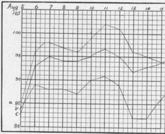
FIG. 10.—The warm wave of August, 1900, at—(a) Charlotte Hall, (b) Grantsville, (c) New Market.
