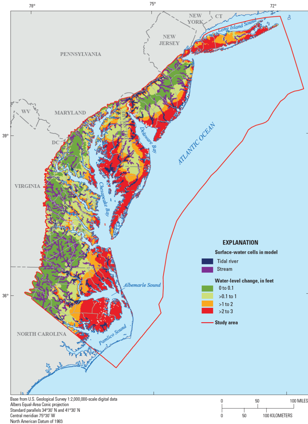
Figure 4. Model-simulated increase in water levels in the surficial aquifer in response to a 3-foot increase (expected by 2100) in the current sea level position across the Northern Atlantic Coastal Plain aquifer system. 125
