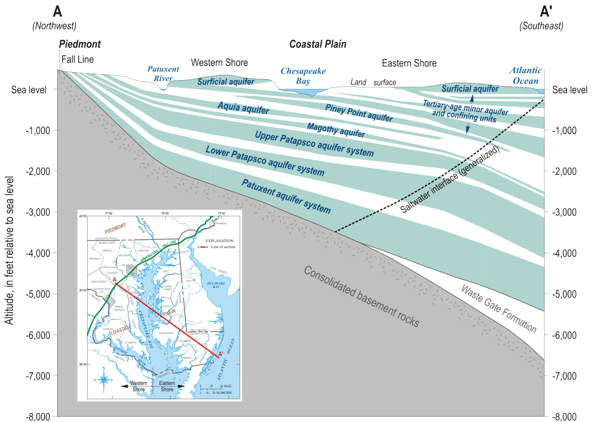
Figure 1. Unconfined (surficial) and Confined Aquifers in Maryland's Coastal Plain. 21
