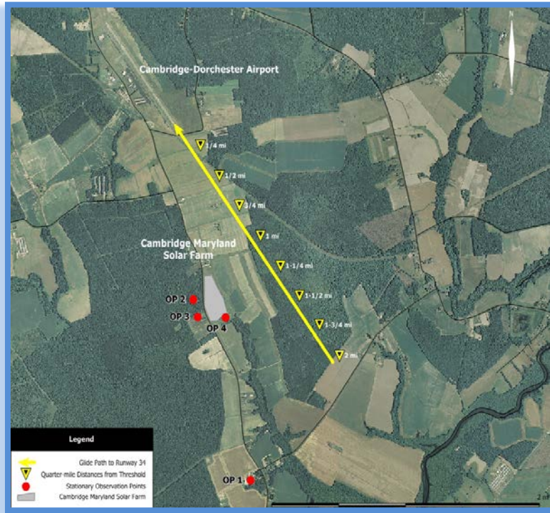
Figure 4-30 SGHAT Stationary Observation Points and Glide Path at Cambridge Maryland Solar Project
