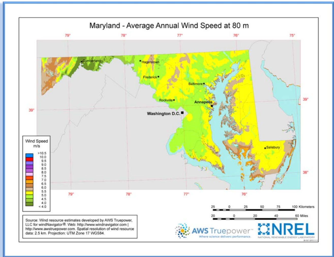
Figure 2-7 Maryland Potential Wind Resources
