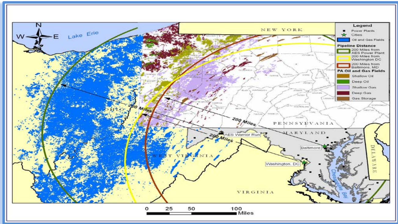
Figure 5-14 Regional Oil and Gas Fields
