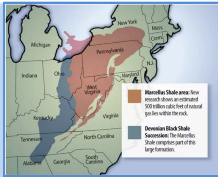
Figure 5-9 Location of the Marcellus Shale Formation
