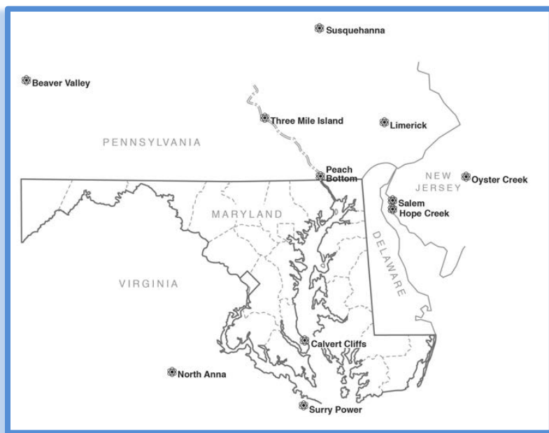
Figure 4-33 Nuclear Power Plants in and Around Maryland
