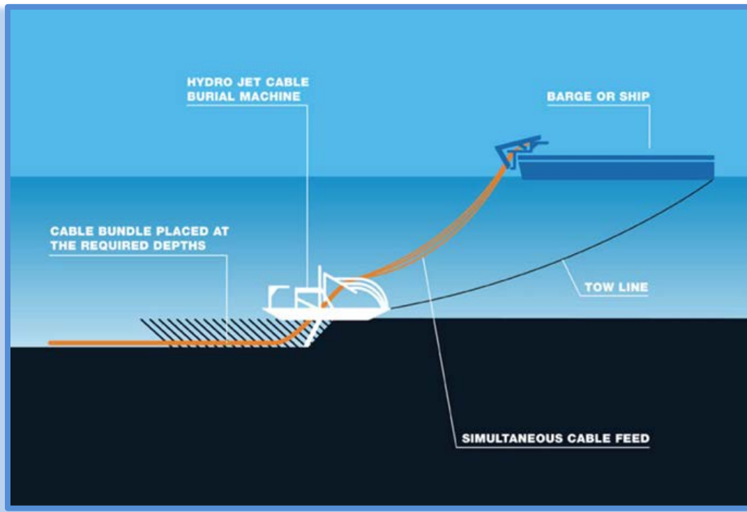
Figure 4-22 Illustration of an Underwater Cable Installation Using Jet Plow Technology
