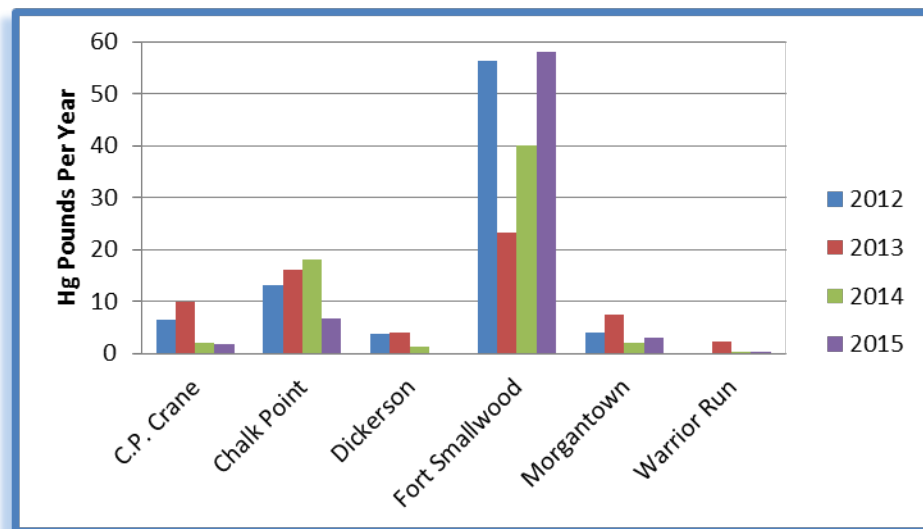
Figure 4-8 Annual Mercury Emissions from Coal-fired Power Plants in Maryland
