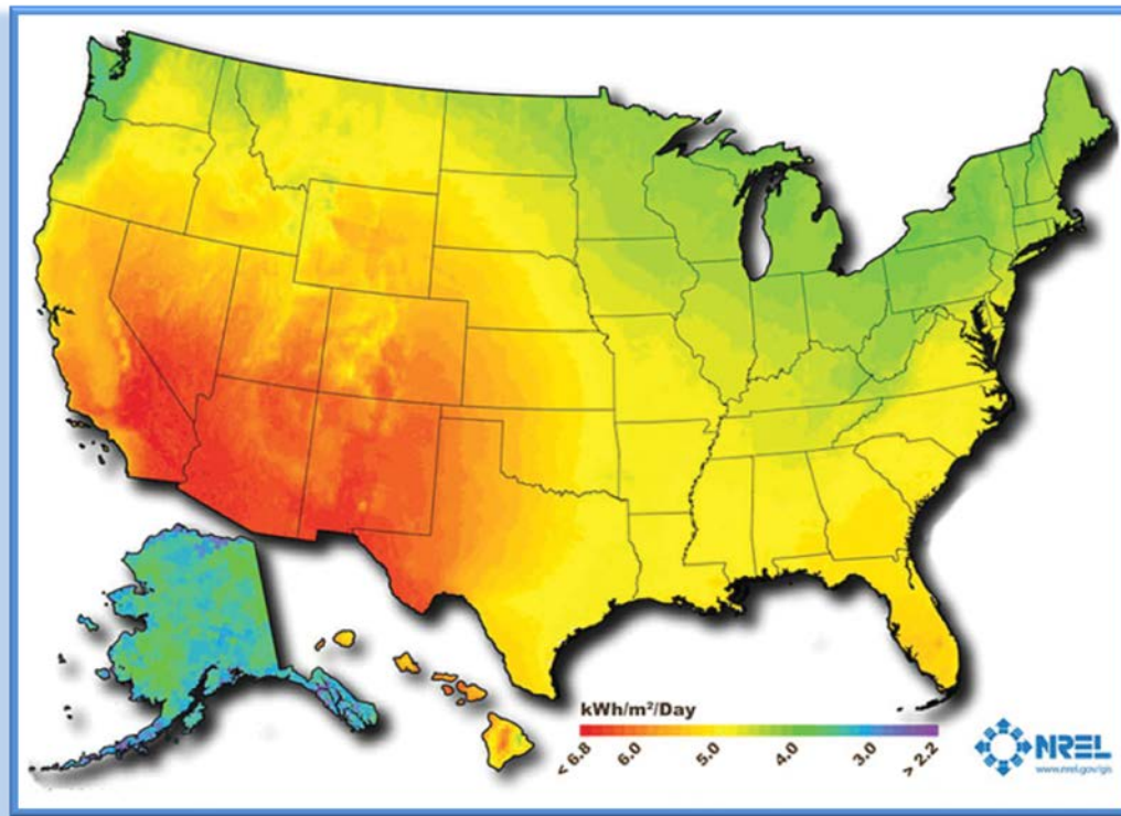
Figure 2-9 Quality of Photovoltaic (PV) Resource
