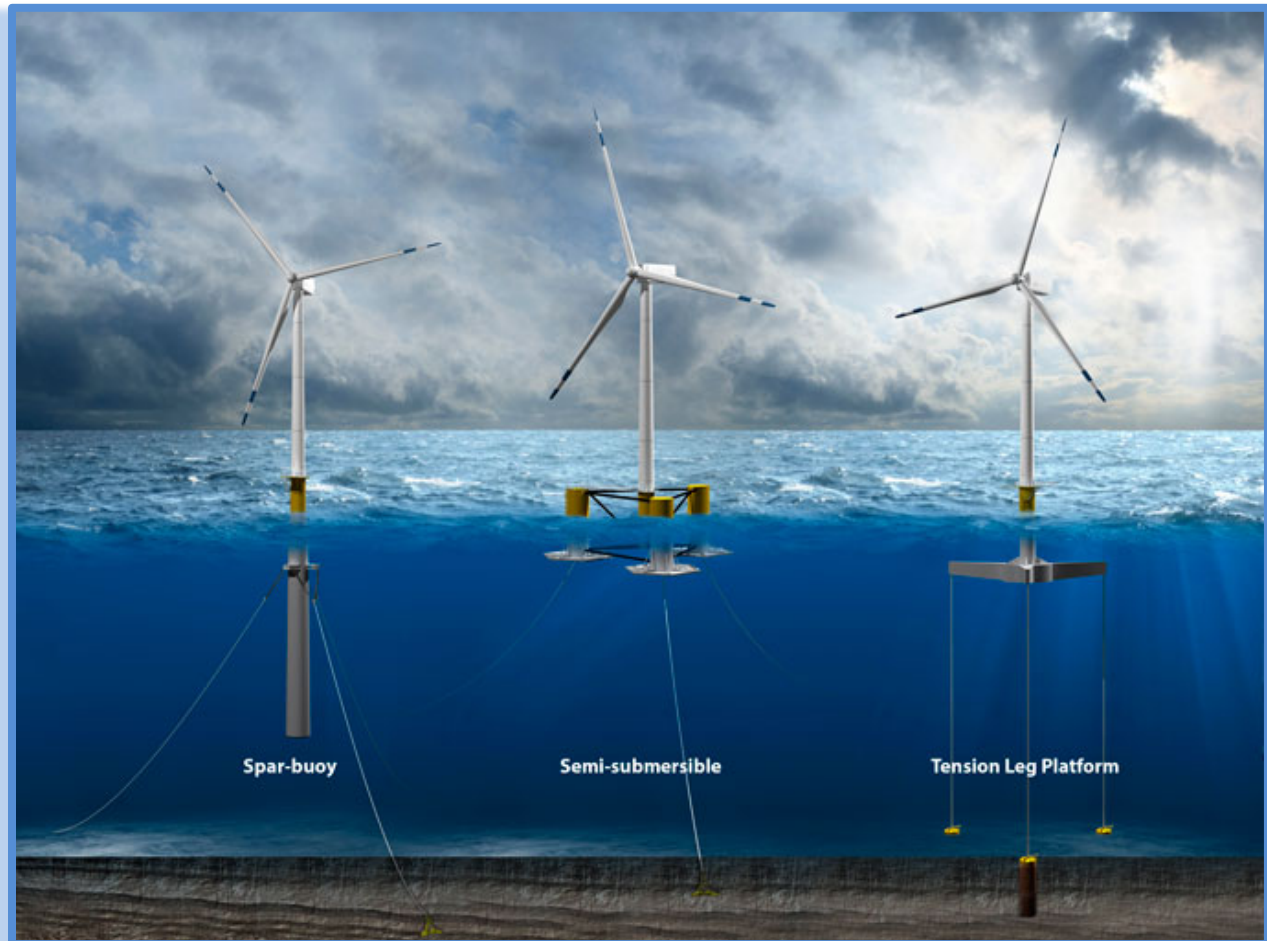
Figure 5-19 Floating Wind Turbine Concepts
