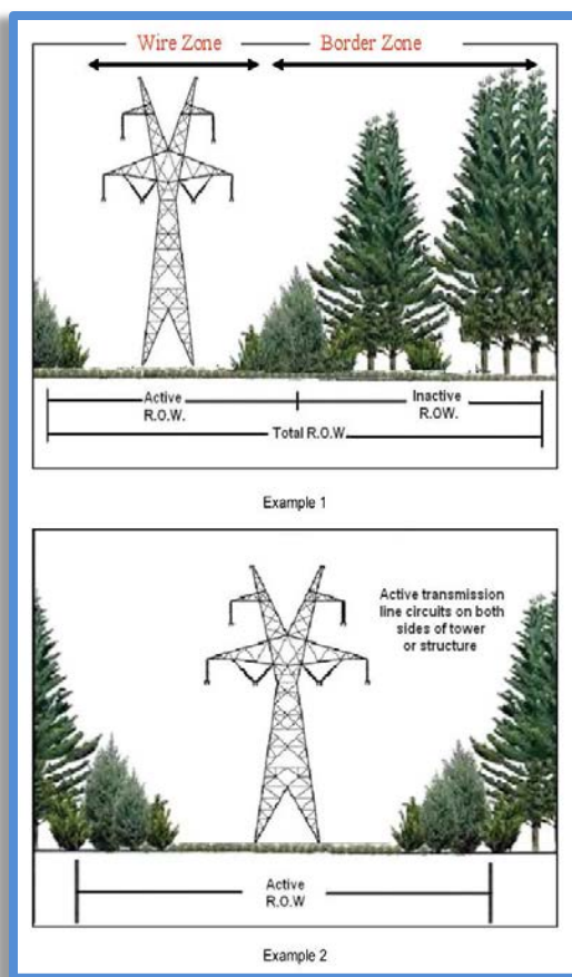
Figure 4-25 Transmission Line Vegetation Management using Feathering Technique
