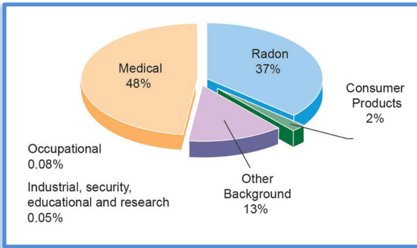
Figure 4-32 Annual Estimated Effective Dose Equivalent (mrem) to the General Population from Natural and Man-Made Sources
