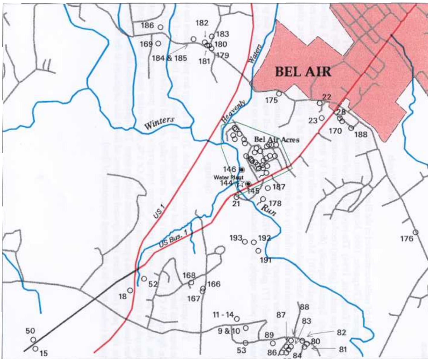
Figure 2.—Locations of inventoryed wells and springs in the vicinity of the Winters Run water plant.
