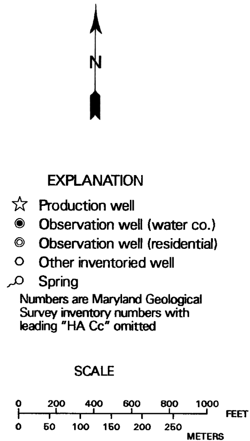
Figure 2.—Locations of inventoried wells and springs in the vicinity of the Winters Run water plant—Continued.
