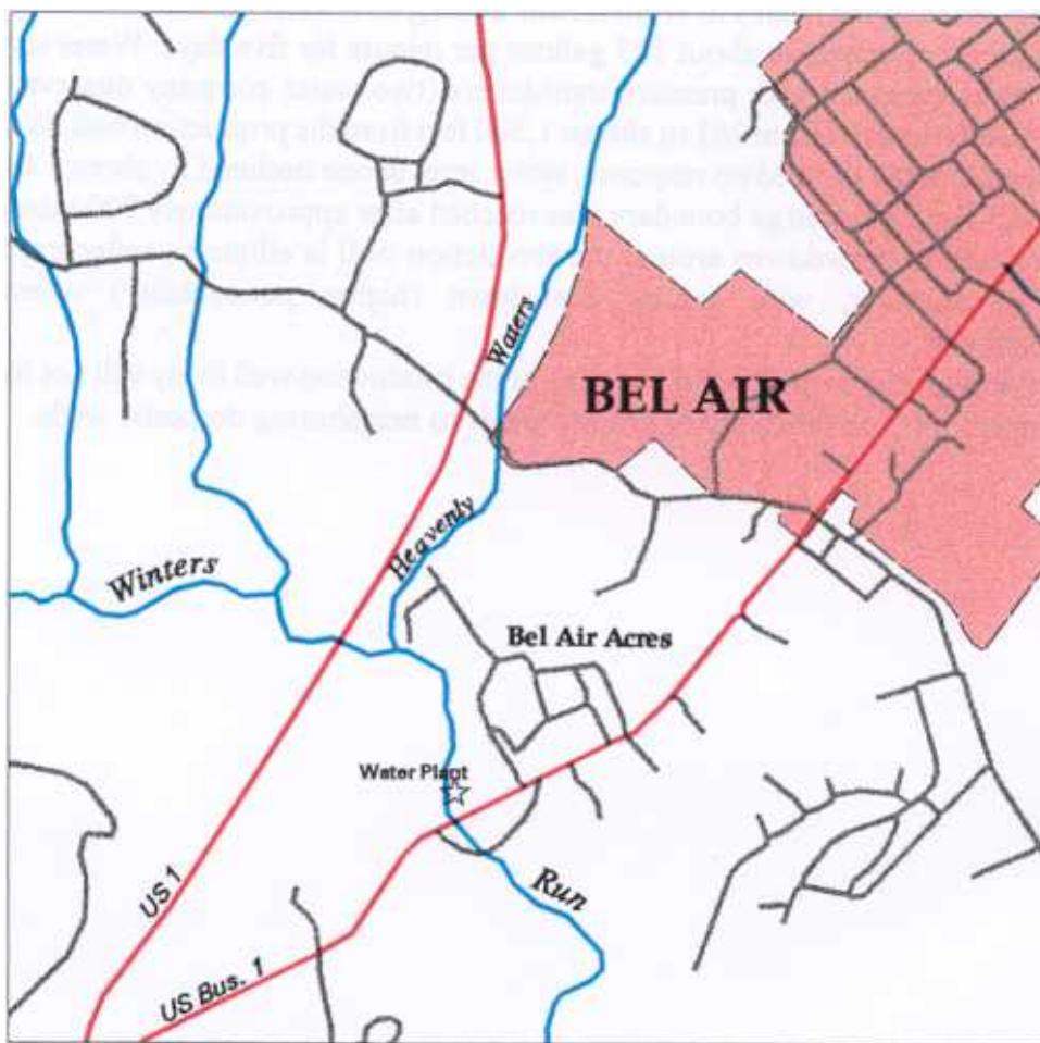
Figure 1.—Location of Winters Run-Bel Air Acres vicinity.
